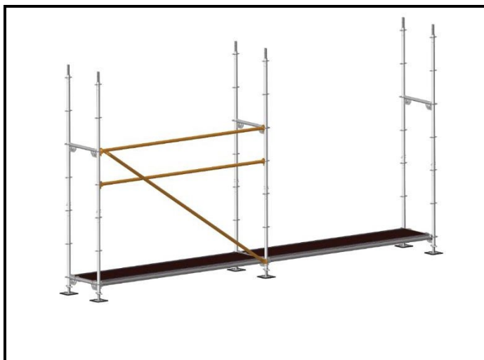
Diagonale SWS-14-XXXX
